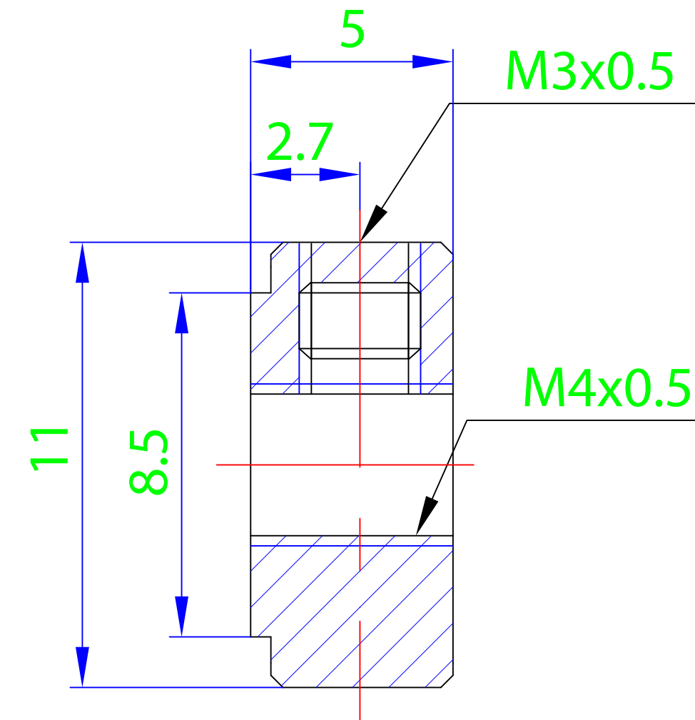
Section X-X
