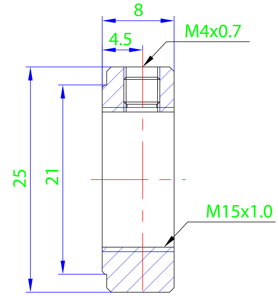
Section X-X
