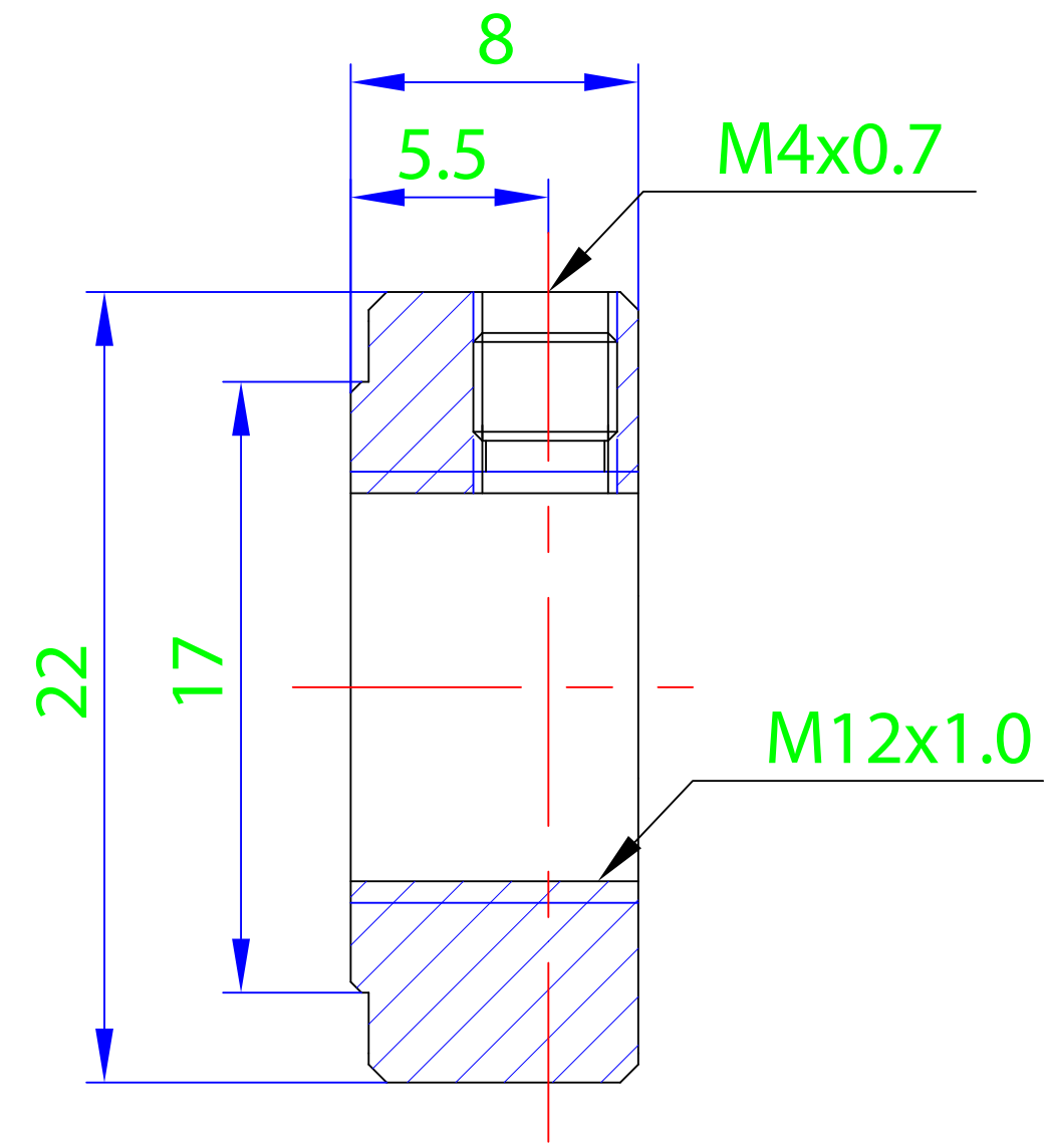
Section X-X
