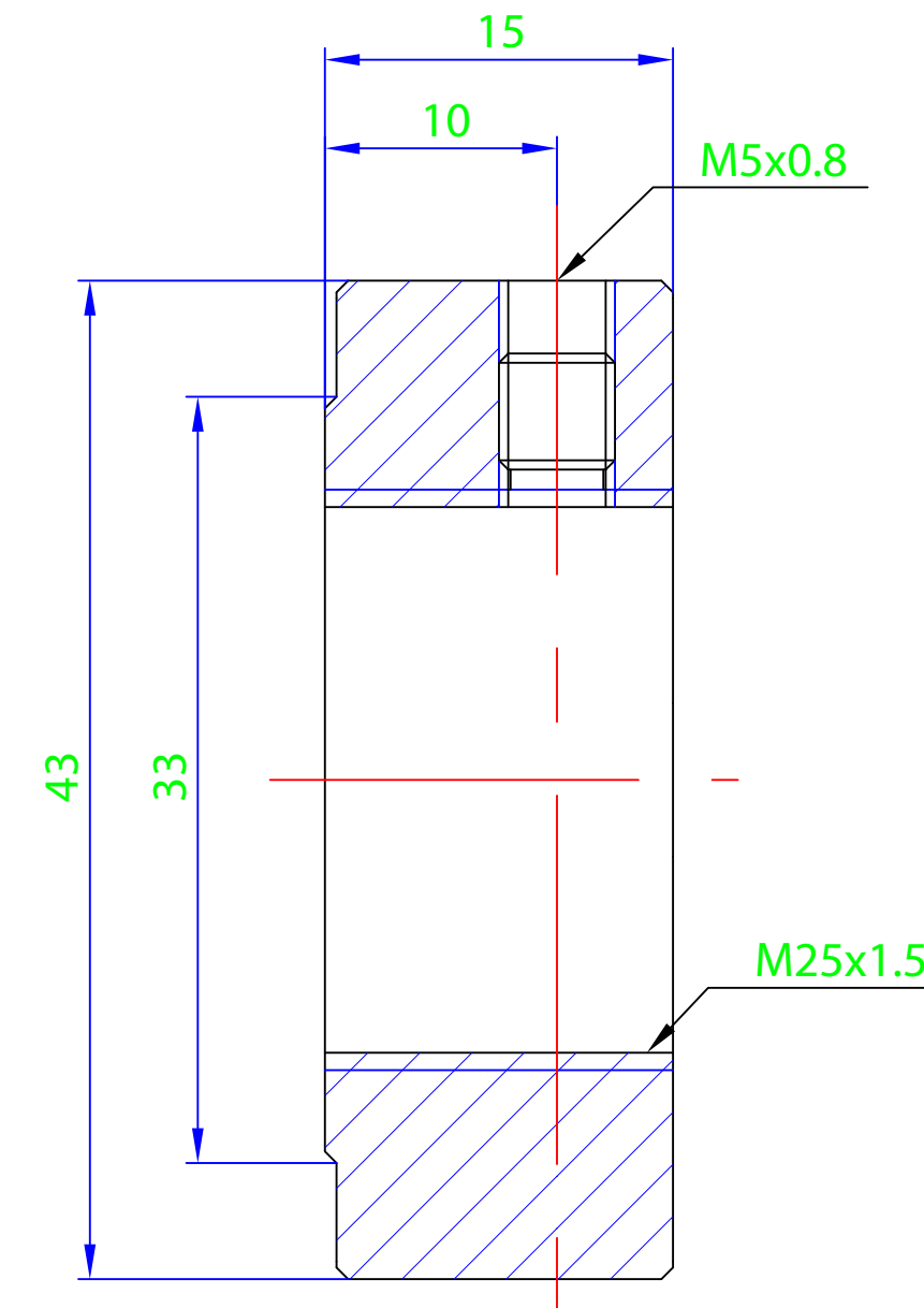
Section X-X
