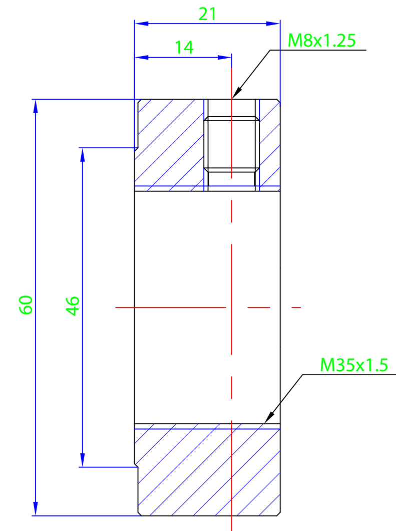
Section X-X
