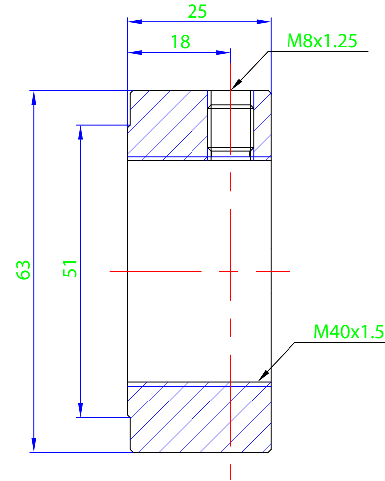
Section X-X
