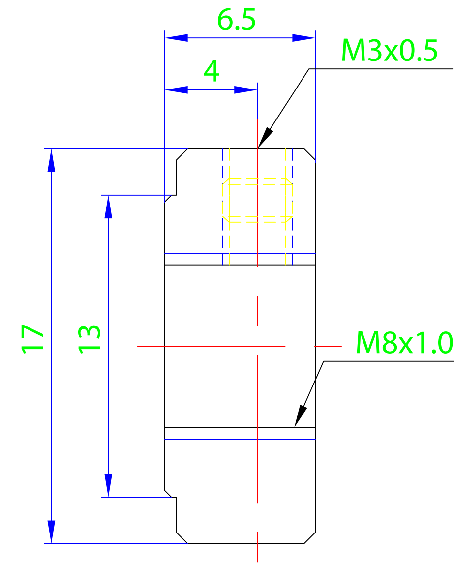
Section X-X
