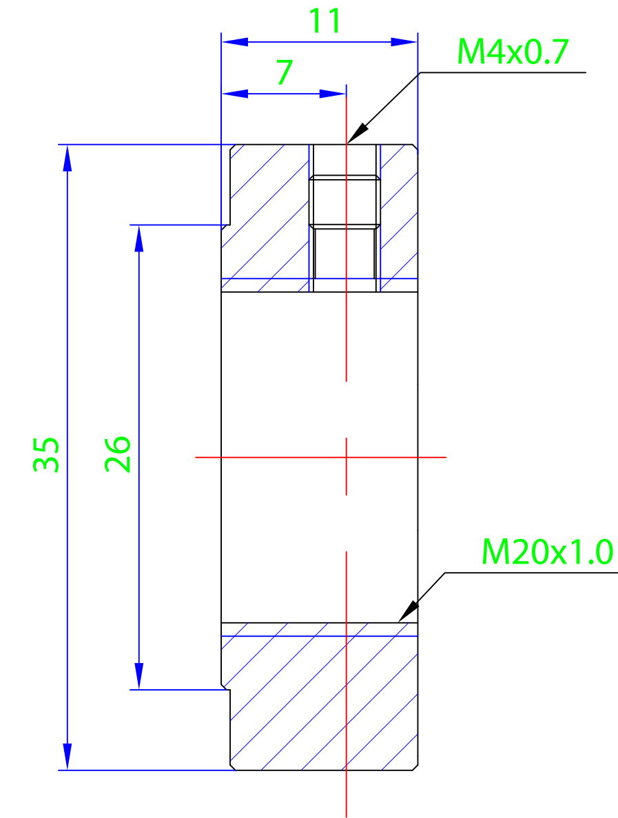
Section X-X
