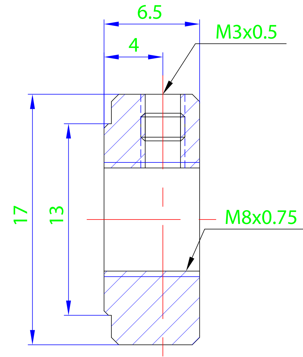
Section X-X
