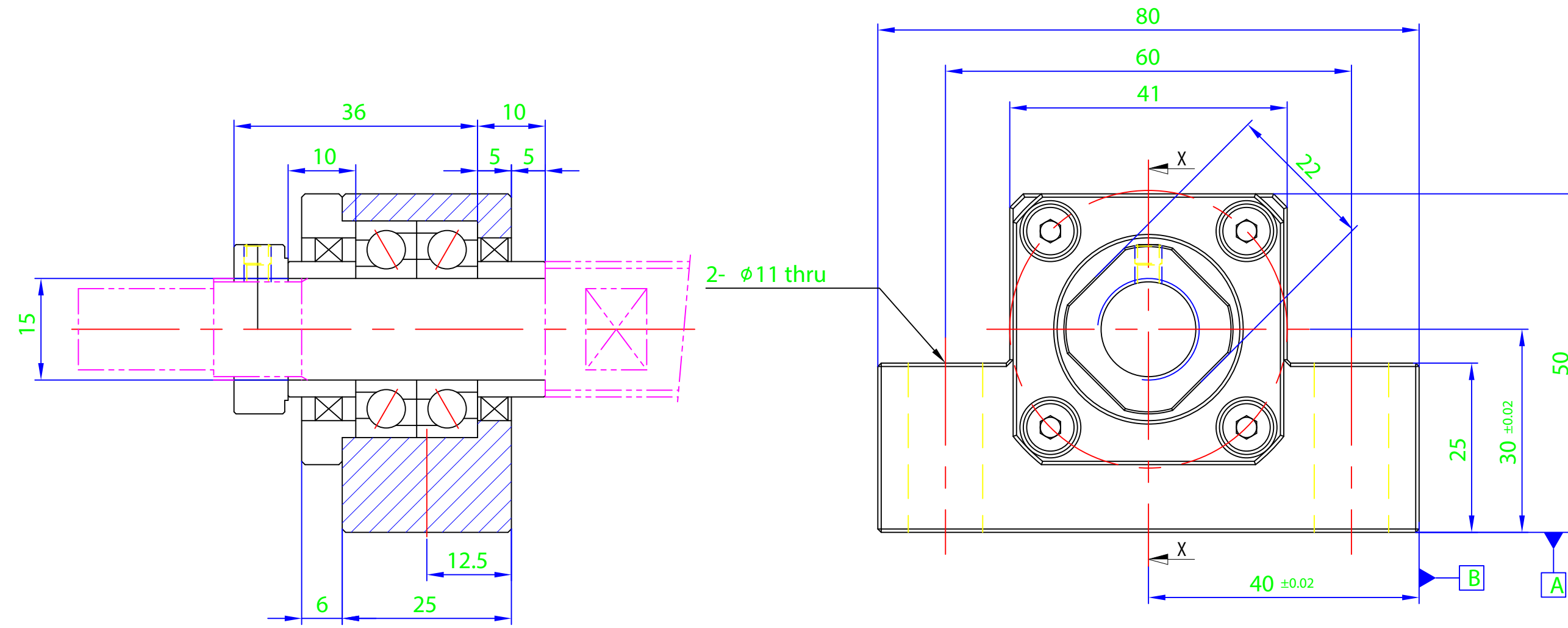
Section X-X
