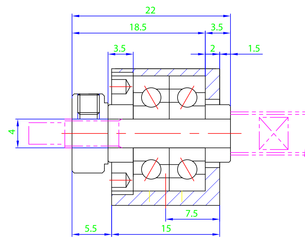
Section X-X
