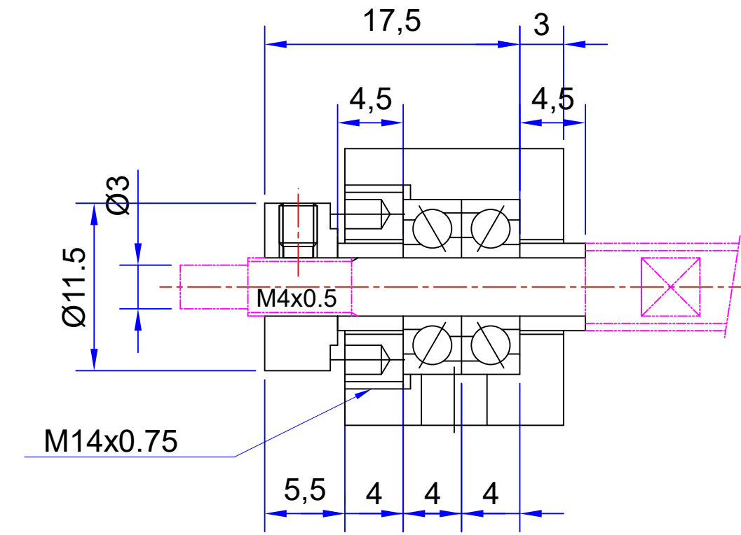
SECTION X-X
