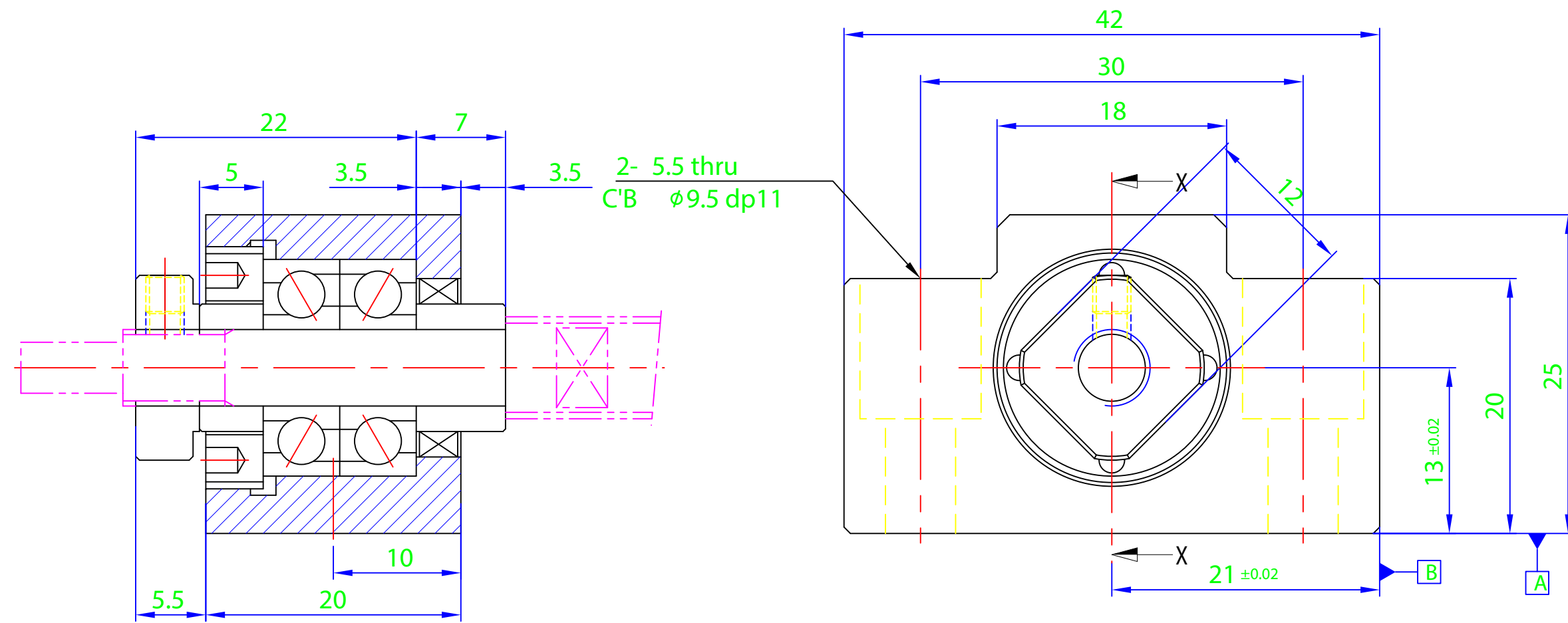
Section X-X
