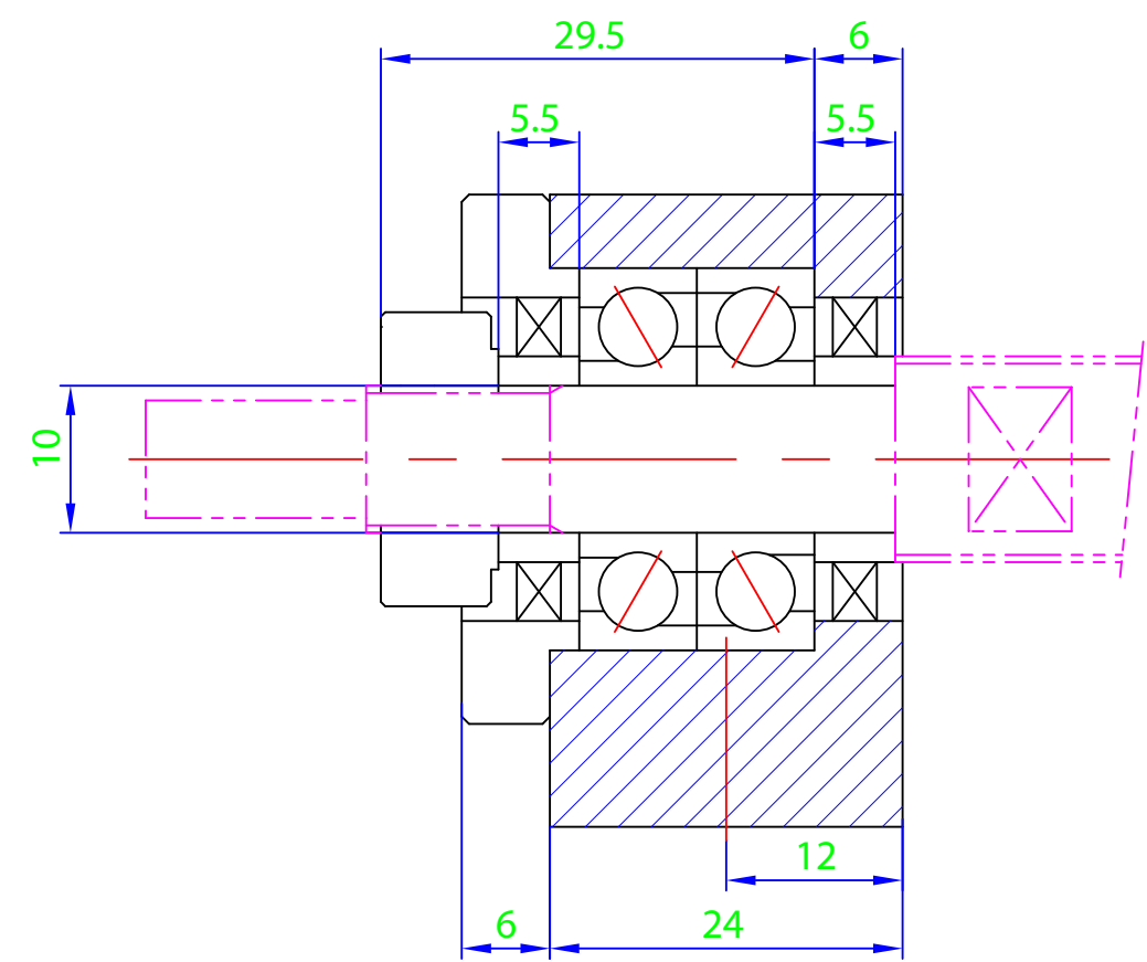
Section X-X
