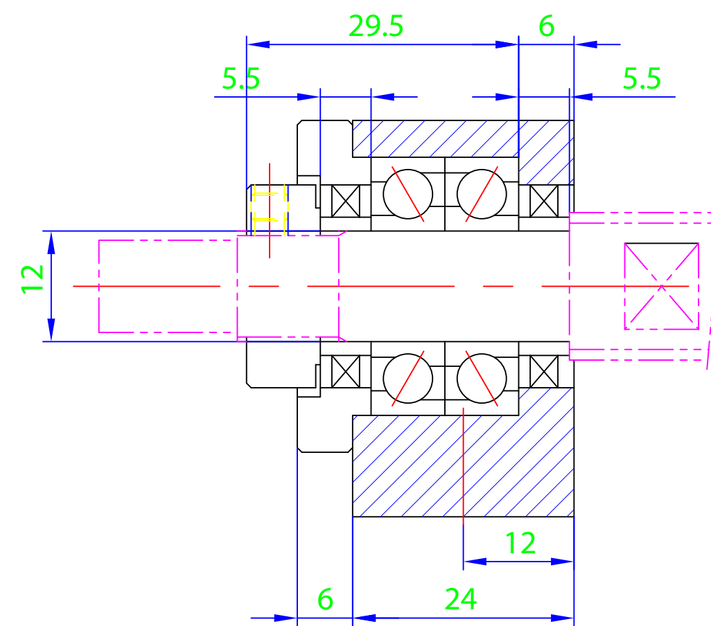
Section X-X
