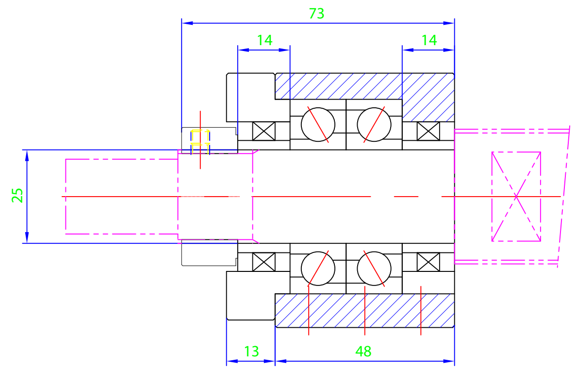
Section X-X
