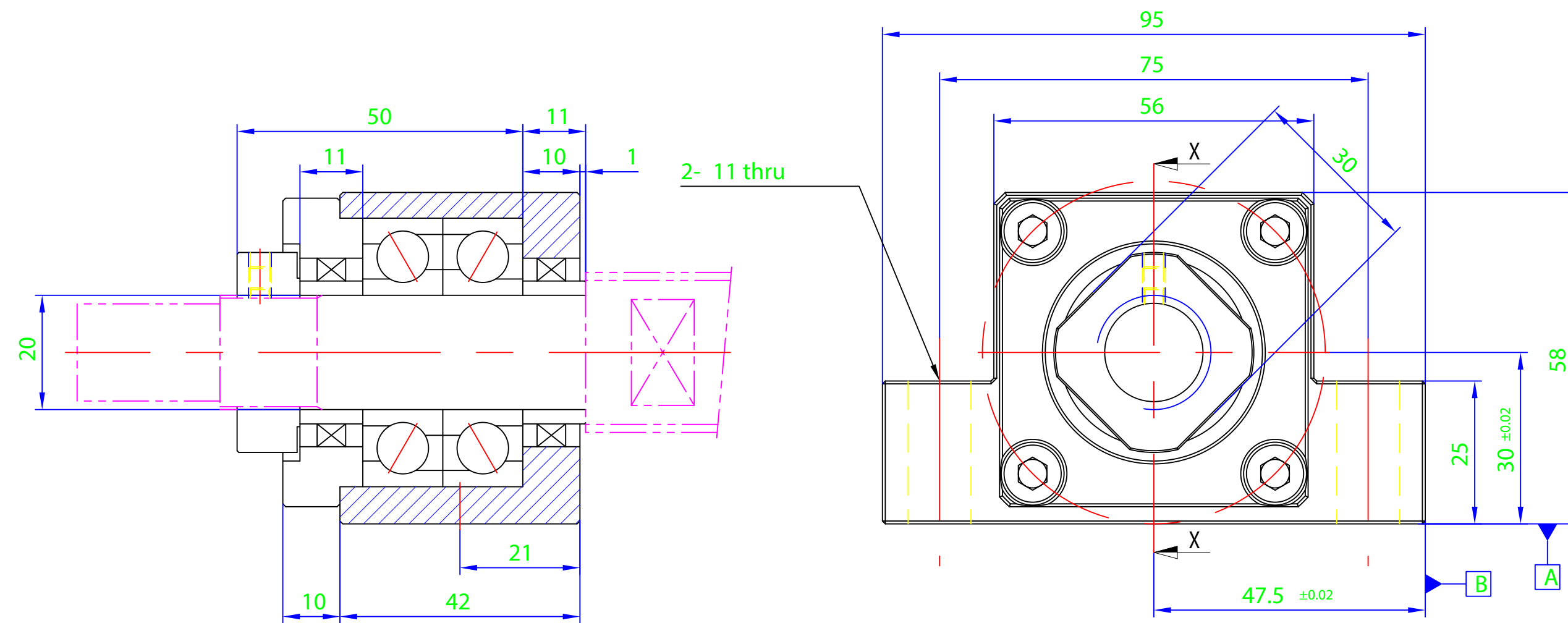
Section X-X
