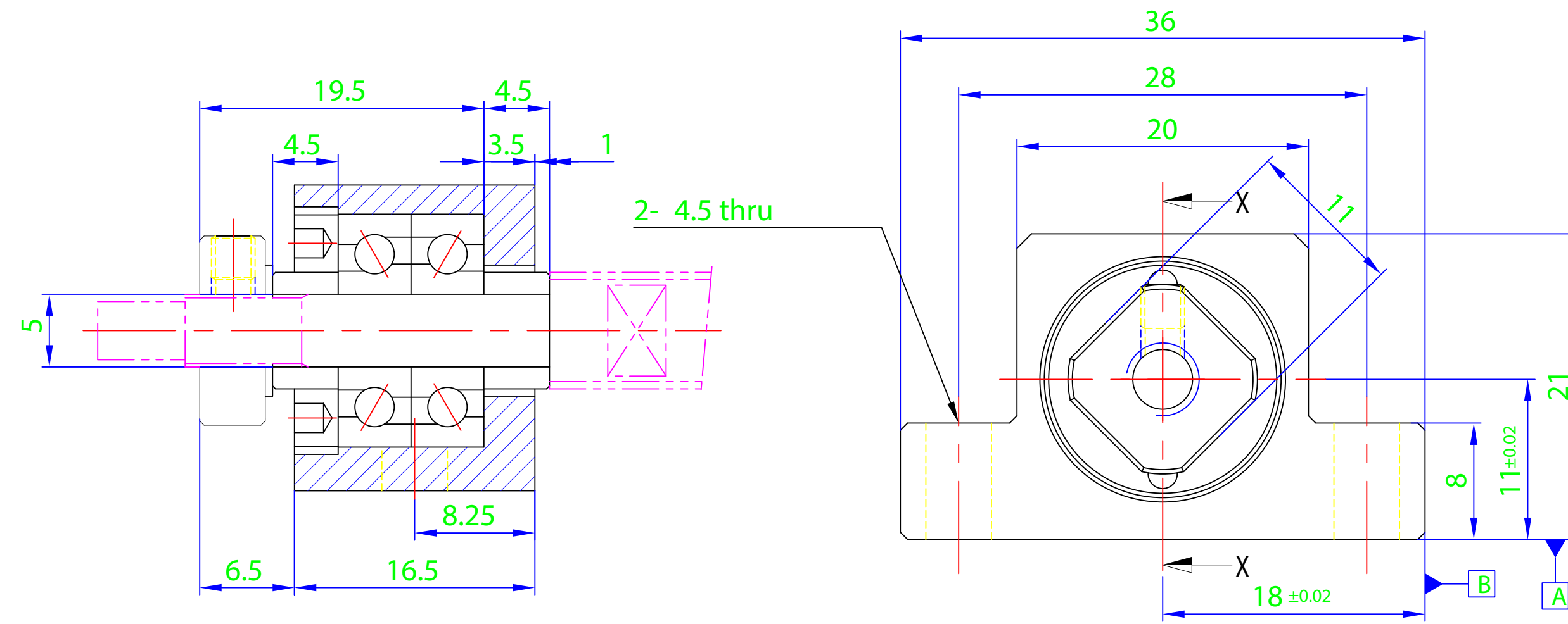
Section X-X
